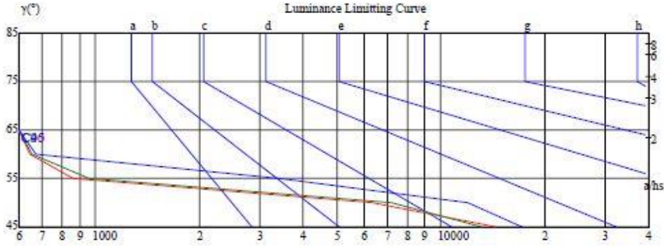
Luminance Limiting Curve
