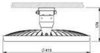
M3 SURFACE MOUNTED
